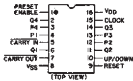
92CS-2701D CD4510B, CD4516B TERMINAL ASSIGNMENT
